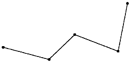
Cassiopeia
