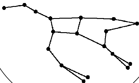
Great Bear
