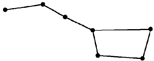
Big Dipper
